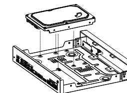
Figure 3-1 Installing hard disk
