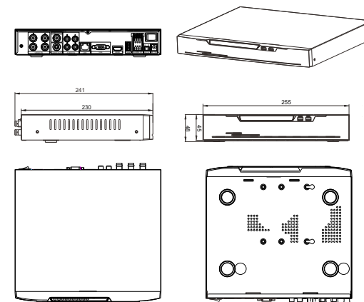
Figure 2-1 Dimensions (Unit:mm)
