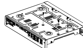
Figure 3-2 Fixing hard disk
